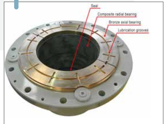
Rudder Bearing
